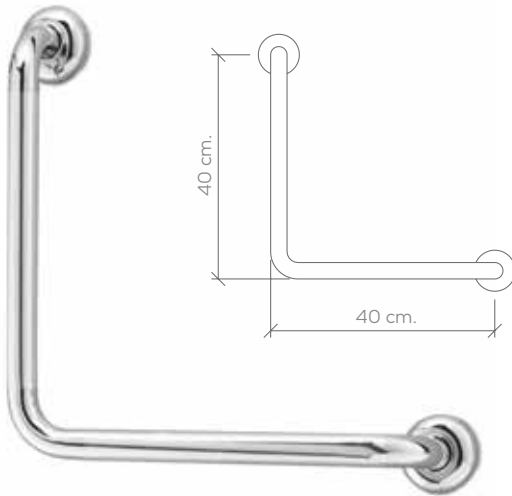
ASIDERO angular 90° Inox. 18/10 18/10 stainless steel 90° angled handrail
