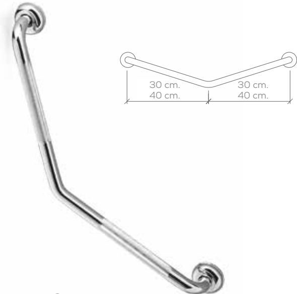
ASIDERO angular 45° Inox. 18/10 18/10 stainless steel 45° angled handrail
