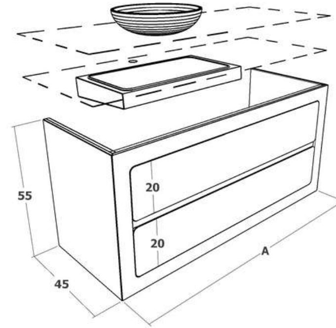
Mueble / bathroom furniture MONOLITH ONYX 55
