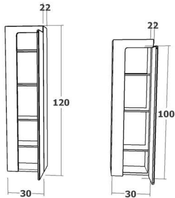
Columna auxiliar / auxiliary column MONOLITH DIAMOND
